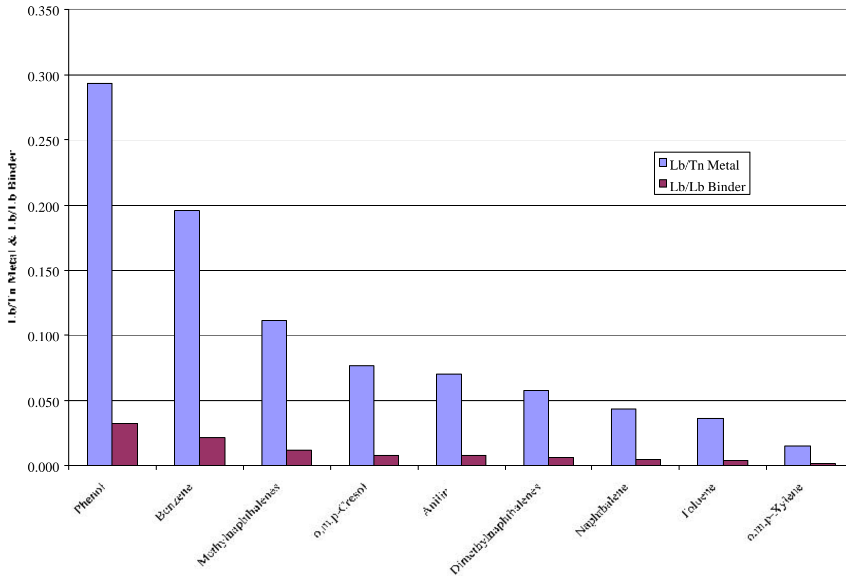
Figure 3-2 Selected HAP Emissions from Test Series EO
