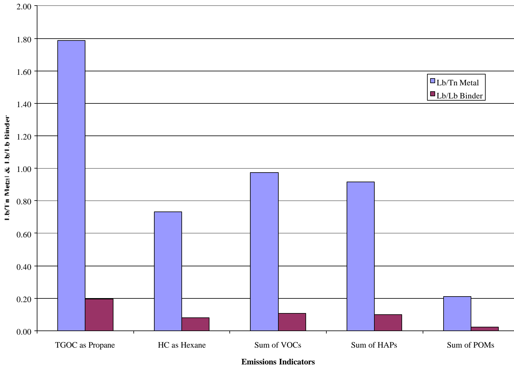
Figure 3-1 Emission Indicators from Test Series EO
