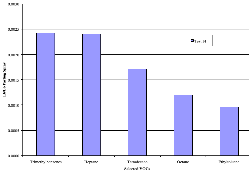
Figure 3-6 Selected VOC Emissions from Test Series FI – Lb/Lb Parting Spray
