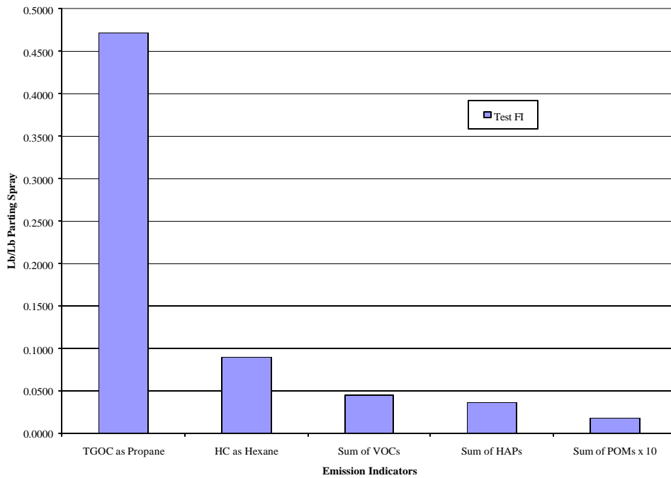
Figure 3-4 Emission Indicators from Test Series FI – Lb/Lb Parting Spray
