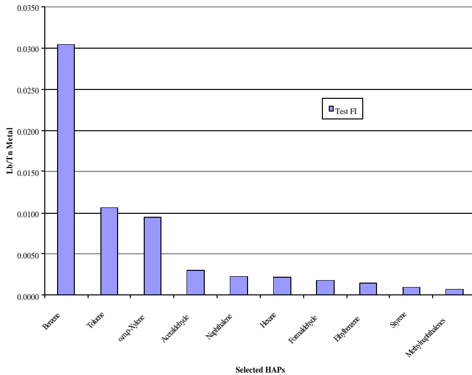
Figure 3-2 Selected HAP Emissions from Test Series FI – Lb/Tn Metal
