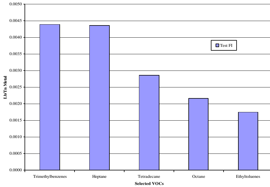
Figure 3-3 Selected VOC Emissions from Test Series FI – Lb/Tn Metal
