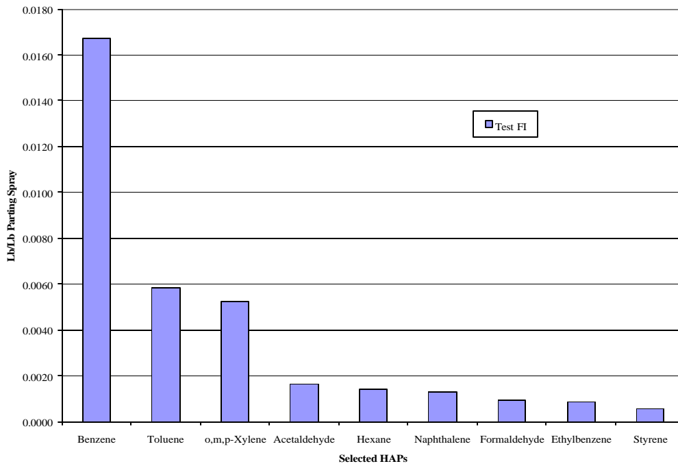
Figure 3-5 Selected HAP Emissions from Test Series FI – Lb/Lb Parting Spray
