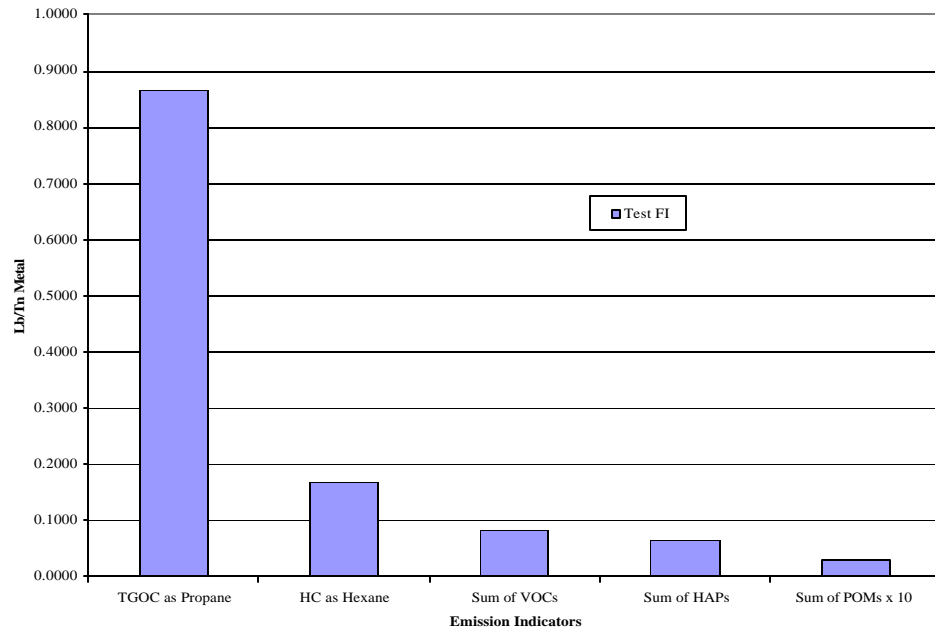
Figure 3-1 Emission Indicators from Test Series FI– Lb/Tn Metal
